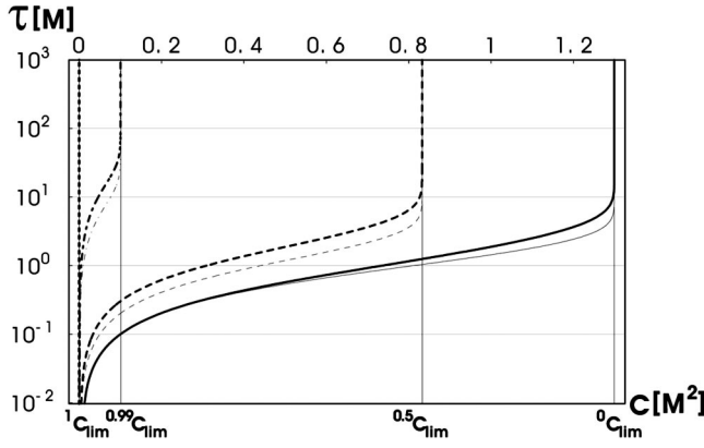
FIG. 1. On a logarithmic scale the time at infinity corresponding to even and zgp boundary conditions, \tau_{even} (gray color) and \tau_{zgp} (black), is shown as a function of the slice label C for the four values of the charge parameter q = Q^2/M^2 being 0 (solid), 0.5 (dashed), 0.99 (dot-dashed), and 1 (dotted). Note that the range 0 \leq C \leq {}^q C_{lim} is getting smaller as {}^q C_{lim} declines from its Schwarzschild value {}^0 C_{lim} = \frac{3}{4}\sqrt{3}M^2 with increasing q such that {}^1 C_{lim} = 0 . The steep gradient in \tau(C) present as C \rightarrow C_{lim} causes numerical problems in finding C for a given time at infinity \bar{\tau} as described in the text.
