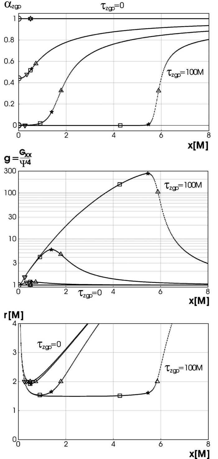
FIG. 3. For zgp boundary conditions numerical results at times \tau_{zgp} = \{0, 1M, 10M, 100M\} are shown to demonstrate the “collapse of the lapse” and “slice wrapping and sucking” taking place as the limiting slice r = 3M/2 is approached. The “symptoms” of slice stretching are the development of a rapidly growing peak in the radial metric function (note the logarithmic scale!) and the outward-drifting of coordinate locations. To study the latter, one should observe the location of the throat, the peak in the radial component of the rescaled 3-metric, and the right-hand event horizon denoted by boxes, stars, and upward pointing triangles, respectively.
